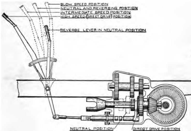
FIG. 254.—Diagram of Control Levers and Transmission of the Packard Car.
